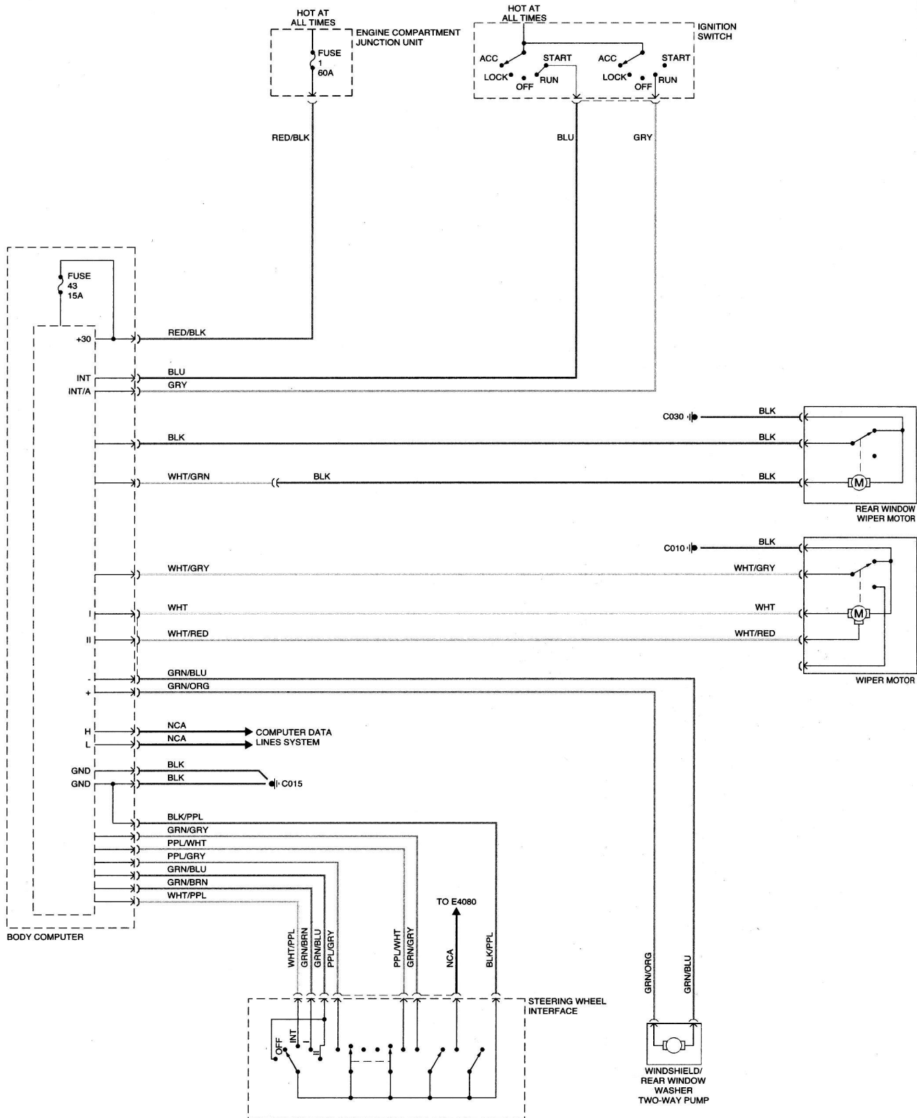
Diagram 9 - Wipers and washers
